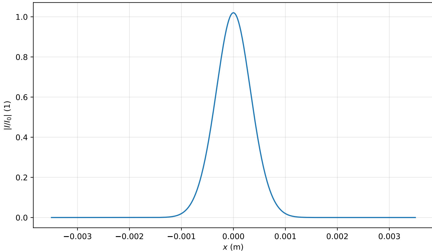
Intensity profile I(x, y = 0, z = 0.478m)/I_0 , P_{in}=0.4P_{cr} , artificial time
